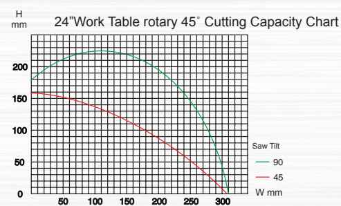
JIH-T5S-30 Worktable Rotary 45° Cutting Capacity Chart
