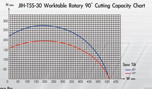
JIH-T5S-30 Worktable Rotary 90° Cutting Capacity Chart
