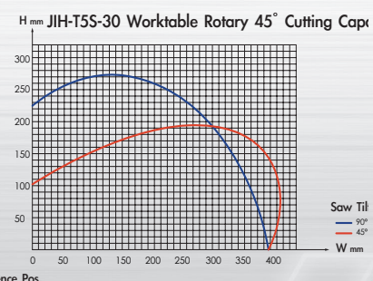
JIH-T5S-30 Worktable Rotary 45° Cutting Capacity Chart
