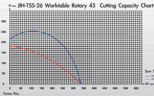
JIH-T5S Cutting Capacity Chart
