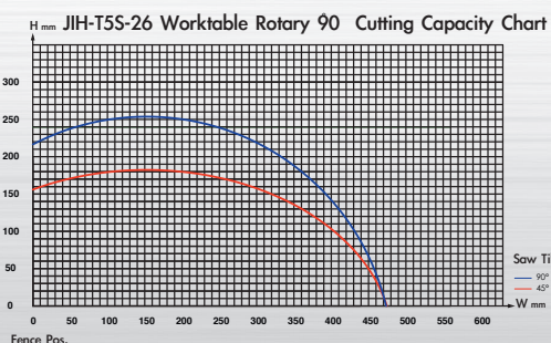
JIH-T5S-26 Worktable Rotary 90° Cutting Capacity Chart
