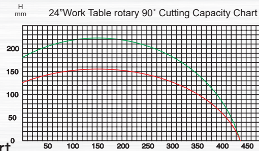
JIH-T5S-26 Worktable Rotary 90° Cutting Capacity Chart
